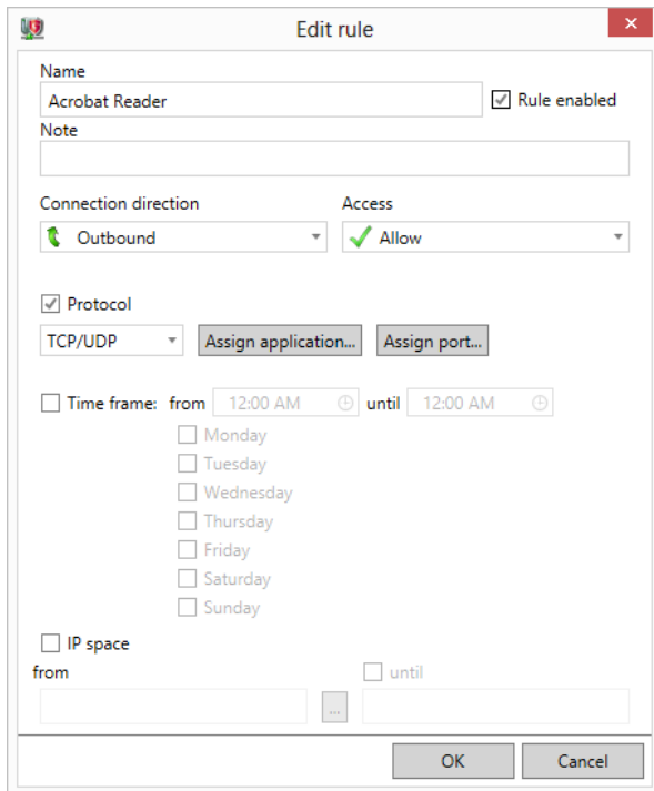
Image 48: G DATA Administrator, Firewall, Rule sets, New rule
