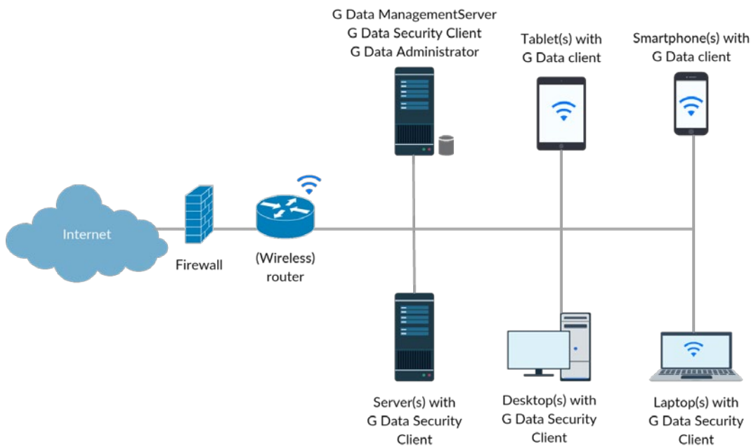
Image 5: Small office network deployment
