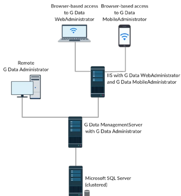
Image 9: ManagementServer deployment with dedicated (clustered) SQL server
