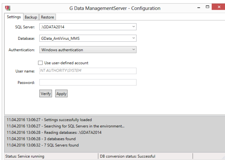
Image 72: GdmmsConfig.exe
