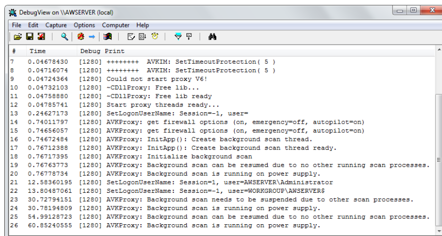
Image 77: DebugView
