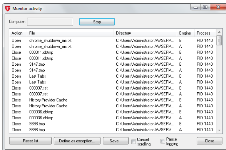
Image 75: Monitor activity
