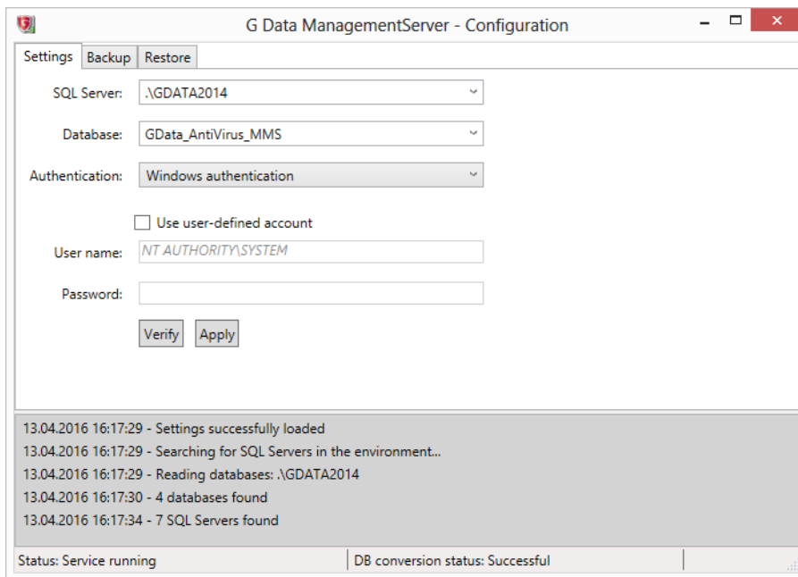
Image 15: GdmmsConfig.exe
