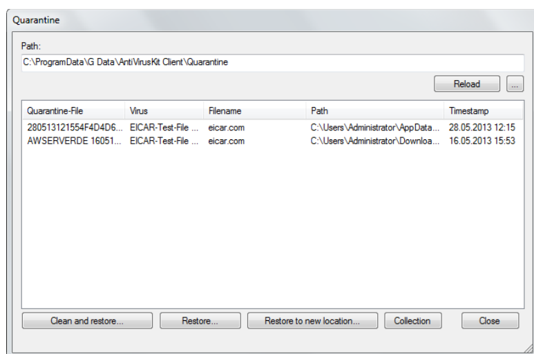
Image 76: Quarantine
