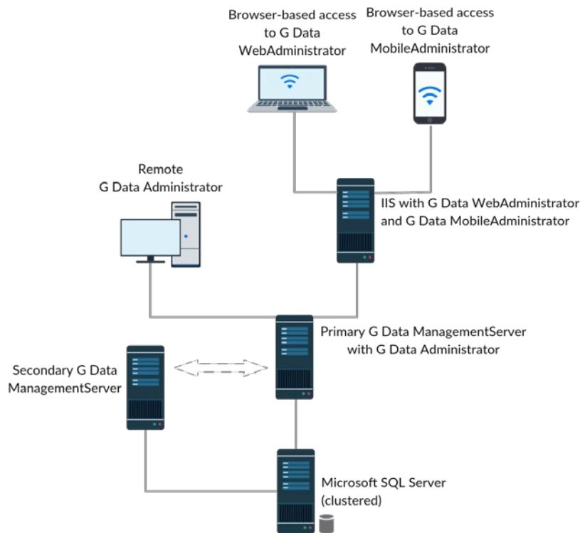
Image 10: ManagementServer deployment with secondary ManagementServer
