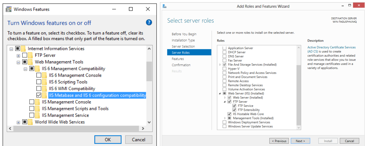
Image 20; 21: Windows 10, Windows Features; Windows Server 2012, Add Roles and Features Wizard
